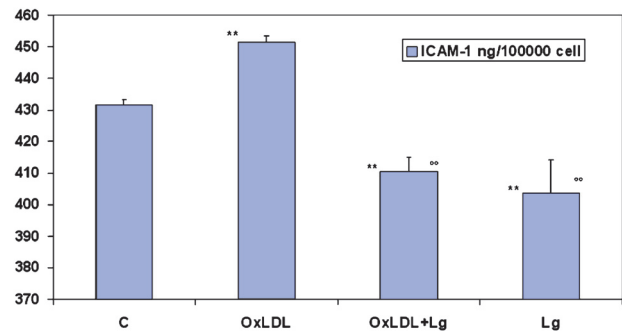
Fig. 2. Effect of oxLDL on endothelial ICAM-1 production. Lisosan G shows a significant reduction of ICAM-1 medium concentration (ELISA method). ** P < 0.01 compared to control; °° P < 0.01 compared to ox-LDL incubation.
